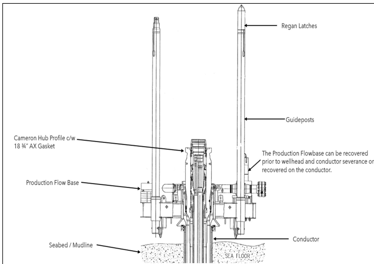
Figure 1.8.1: South Magnus and Magnus Swift Wellhead Design
