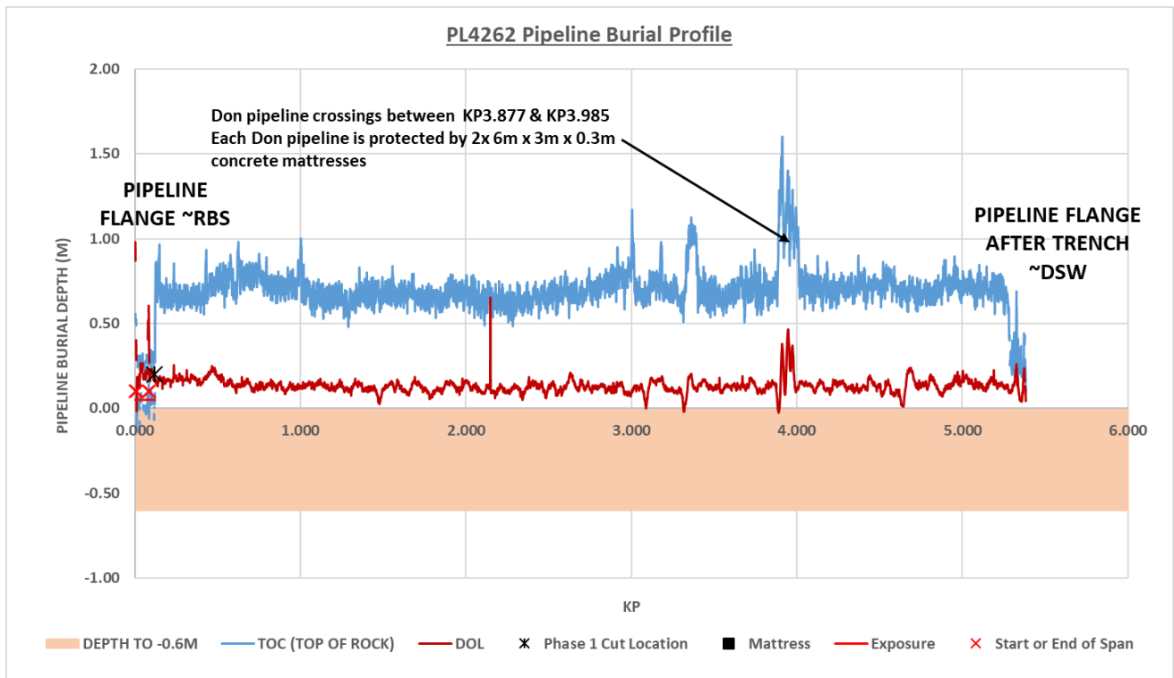
Figure 3.3.12: PL4262 depth of burial profile
