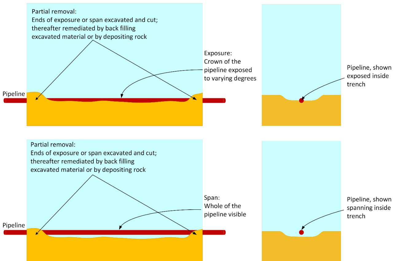
Figure 4.1.1: Exposures, spans & partial removal
