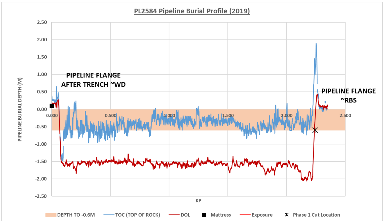
Figure 3.4.8: PL2584 depth of burial profile
