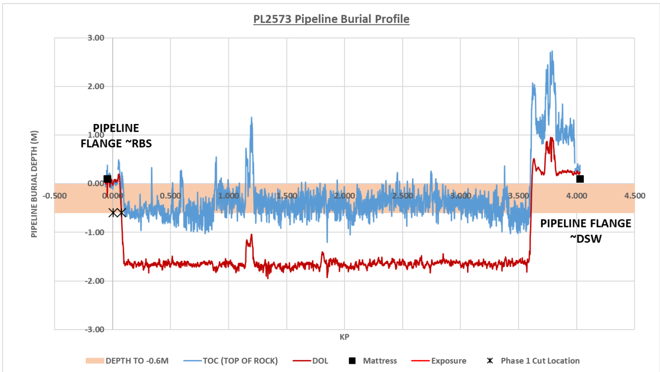
Figure 3.3.4: PL2573 depth of burial profile
