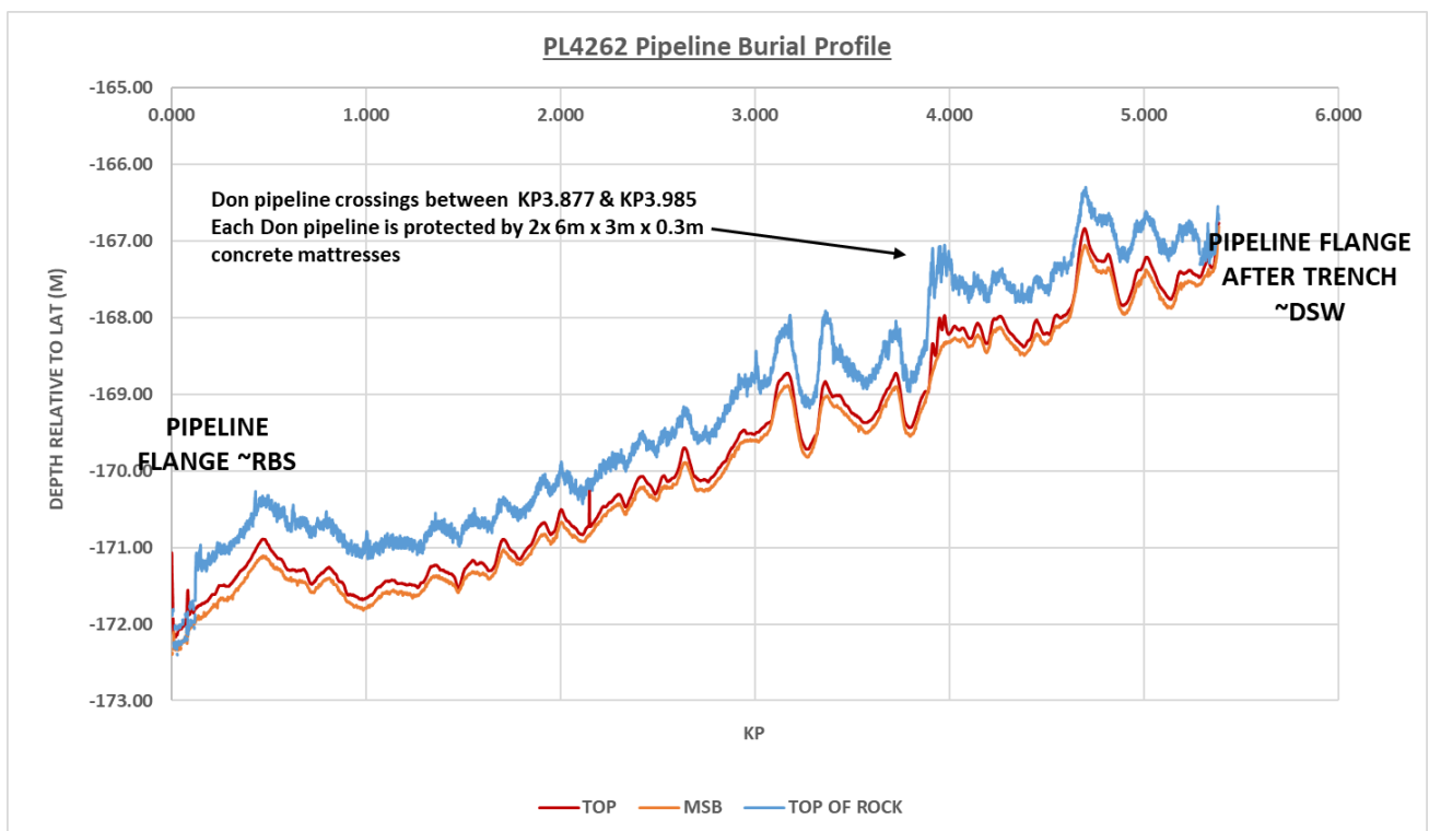
Figure 3.3.11: PL4262 seabed & burial profile
